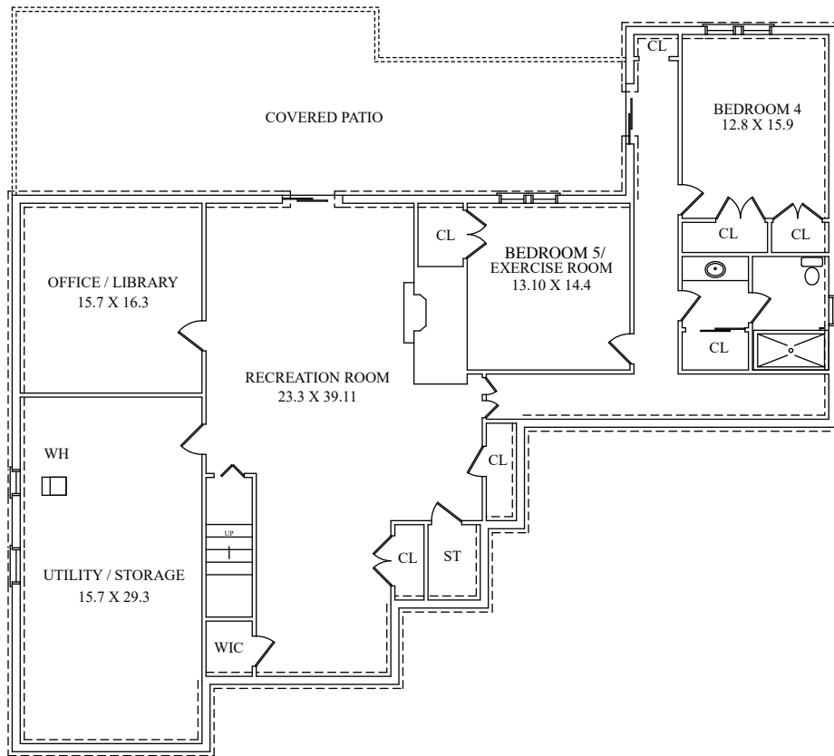
LOWER LEVEL
