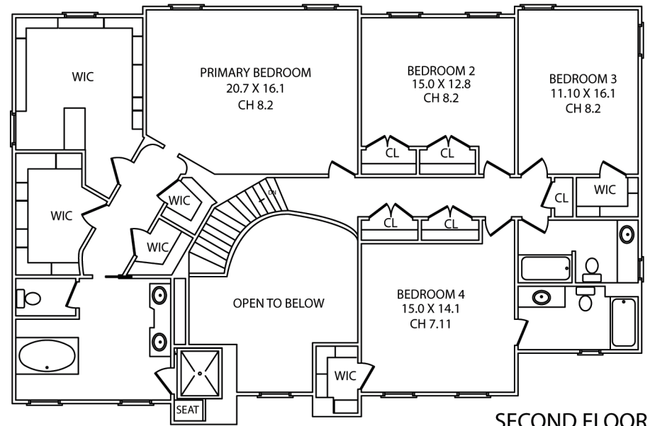
SECOND FLOOR
