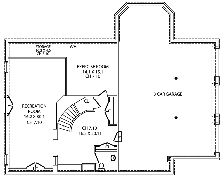
LOWER LEVEL
