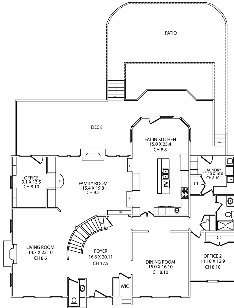
FIRST FLOOR
