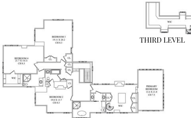
SECOND LEVEL
