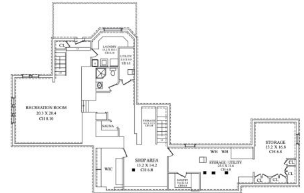
LOWER LEVEL
