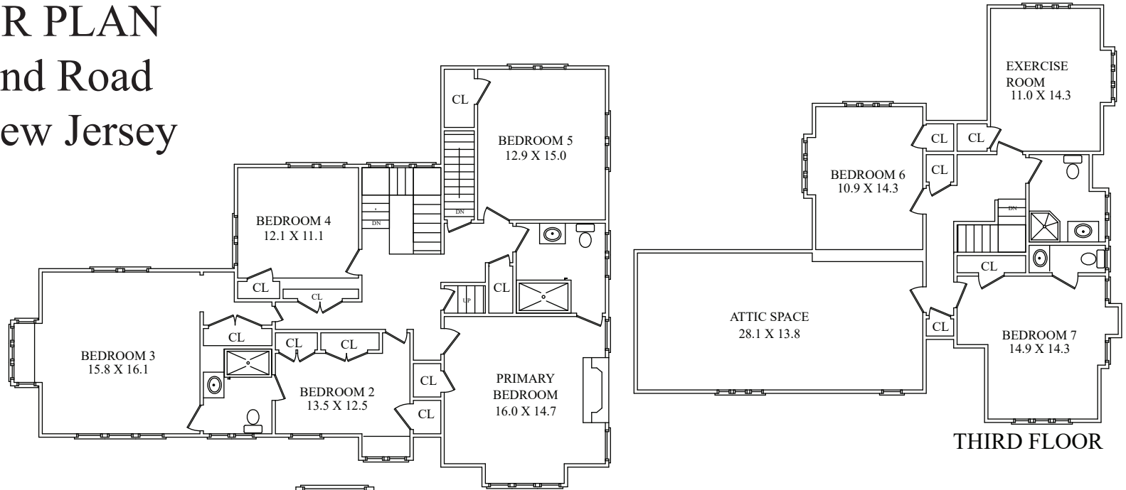
SECOND FLOOR
