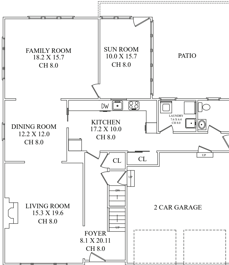
FIRST FLOOR
