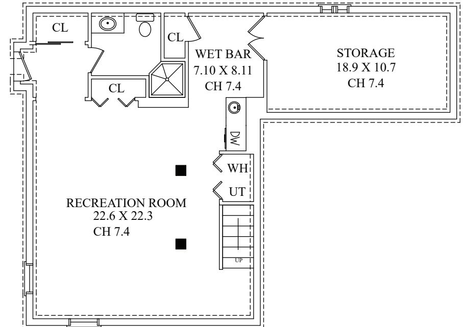
LOWER LEVEL
