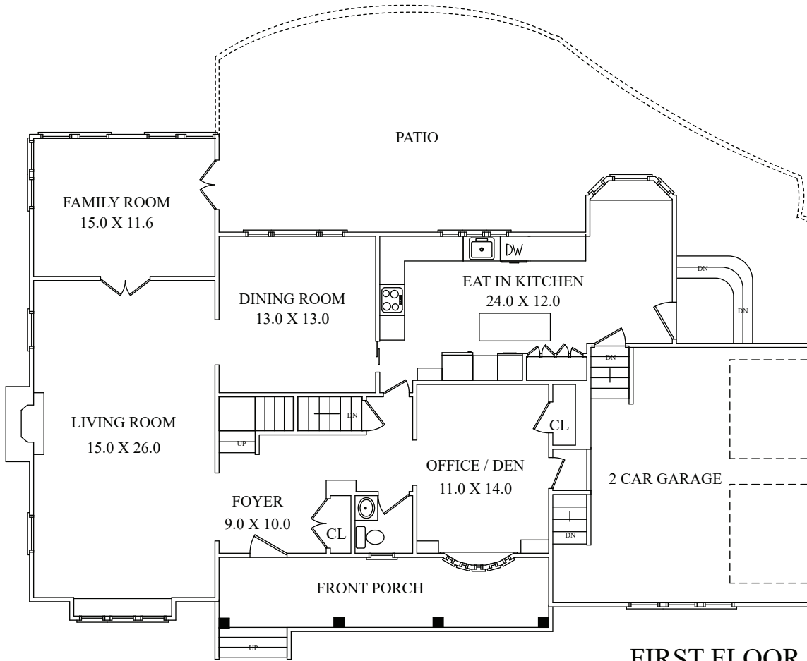
FIRST FLOOR
