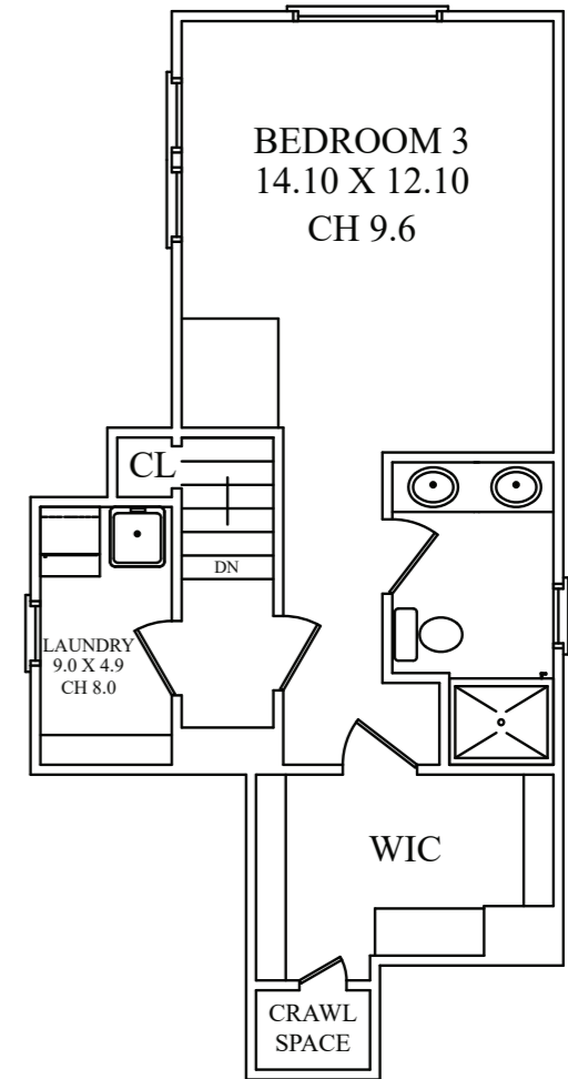
SECOND FLOOR
