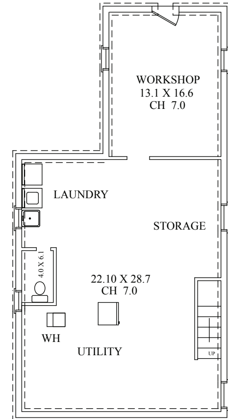
LOWER LEVEL
