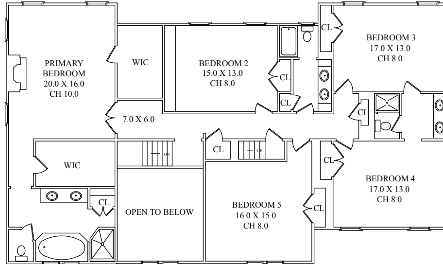
SECOND FLOOR
