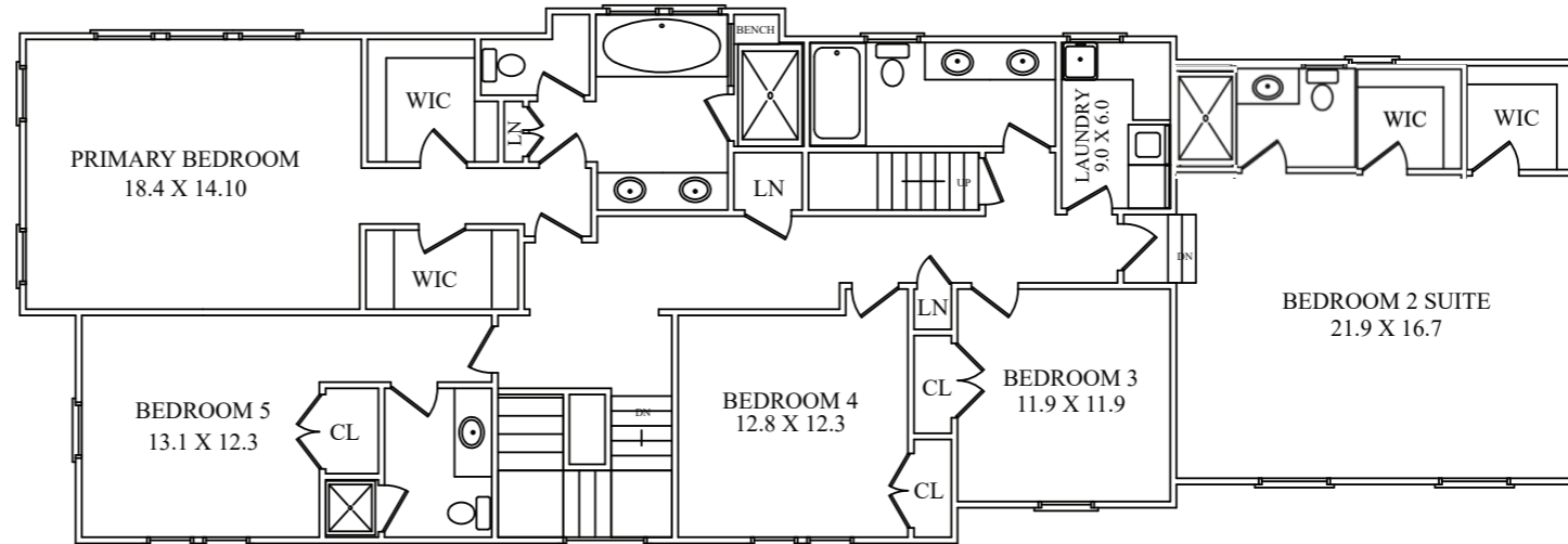
SECOND FLOOR
