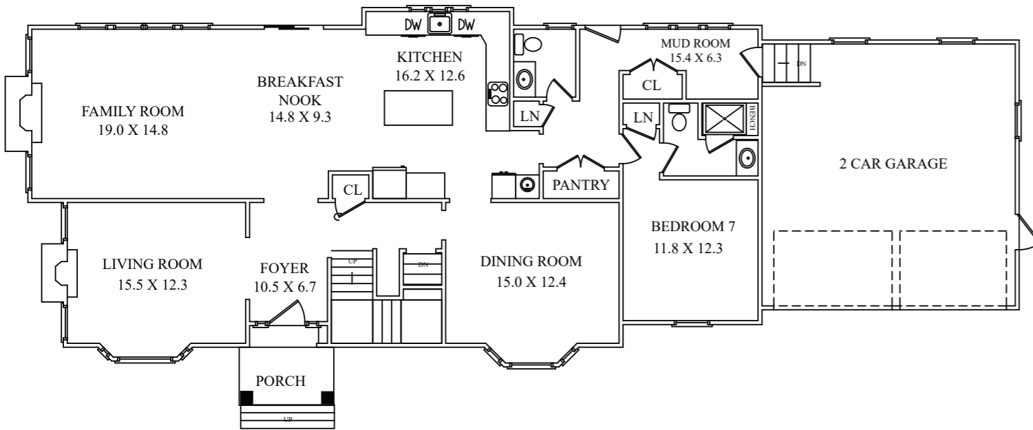
FIRST FLOOR
