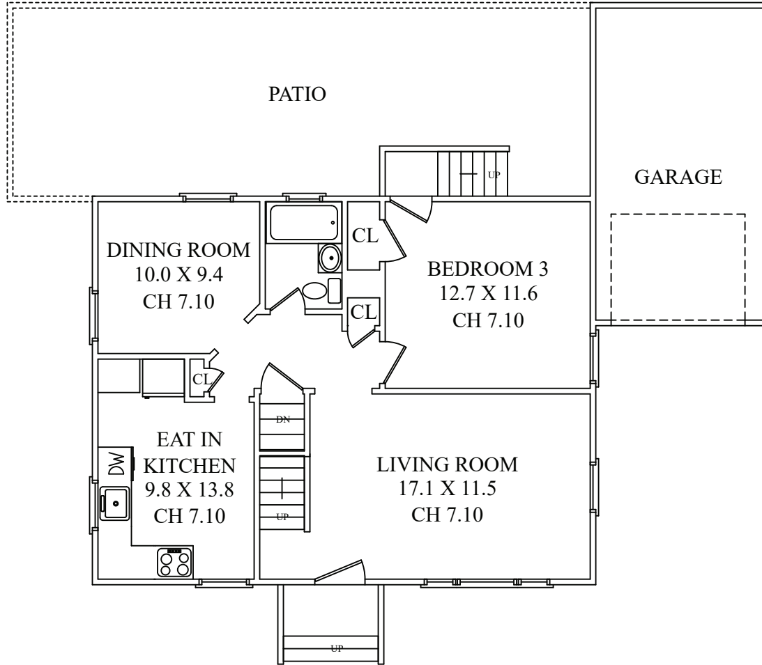
FIRST FLOOR
