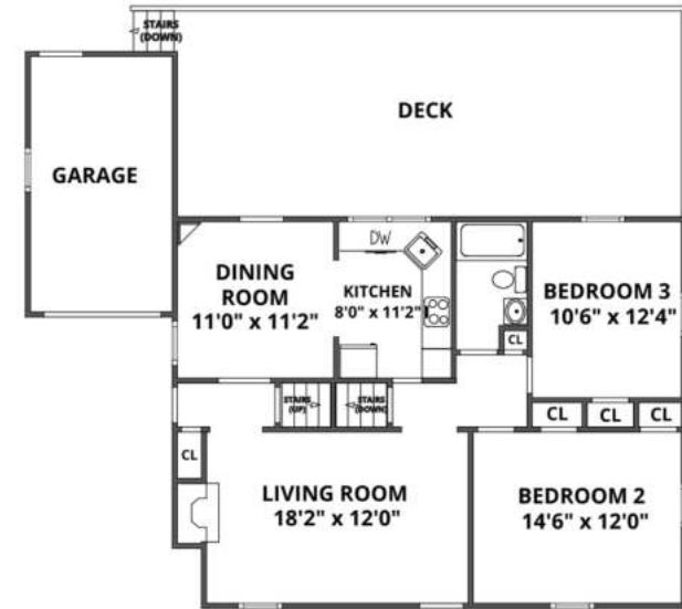
FIRST LEVEL
