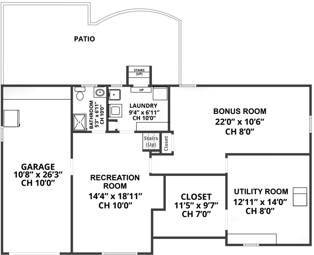
LOWER LEVEL
