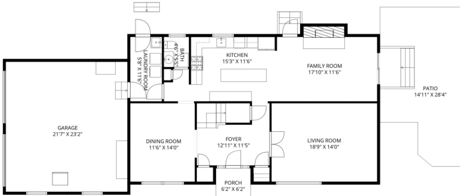
FIRST LEVEL
