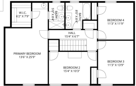
SECOND LEVEL
