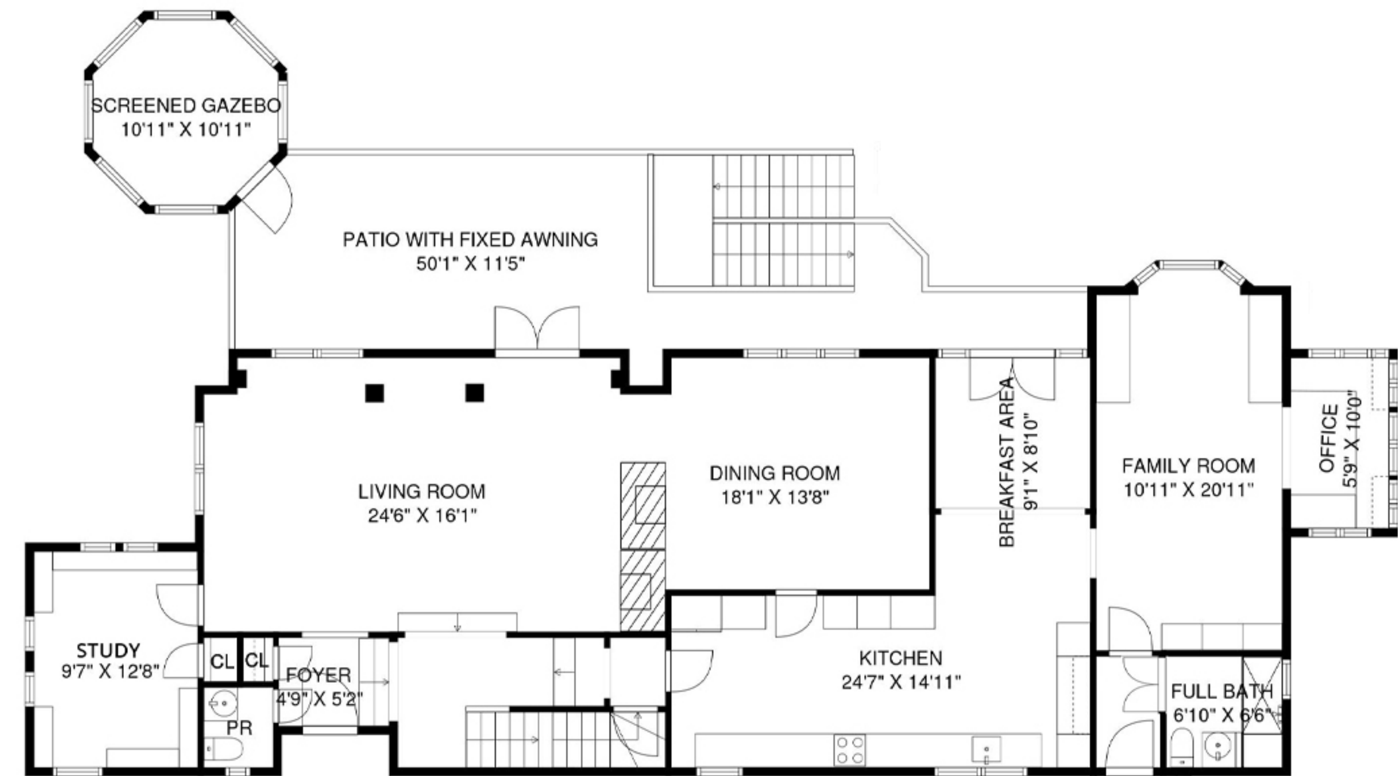
FIRST FLOOR
