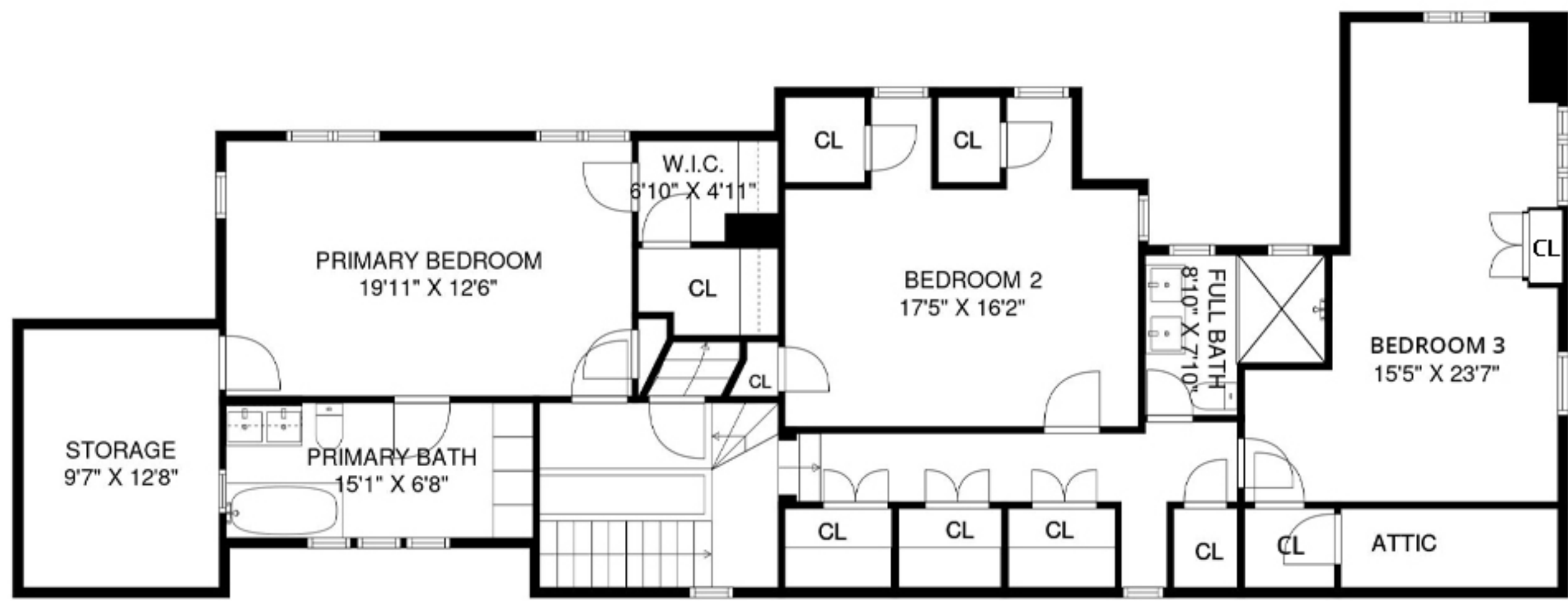
SECOND FLOOR
