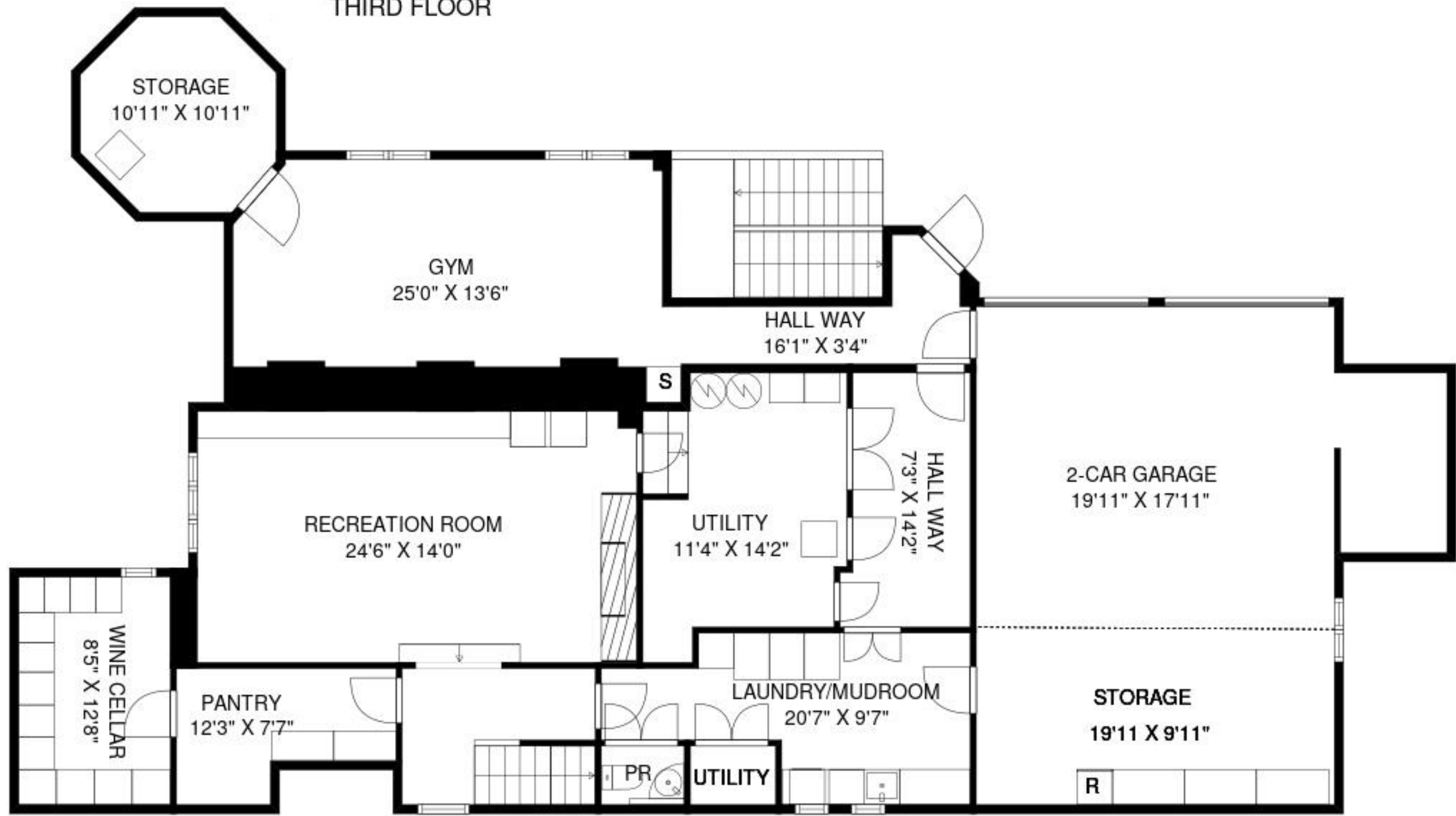
LOWER LEVEL
