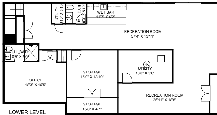
LOWER LEVEL
