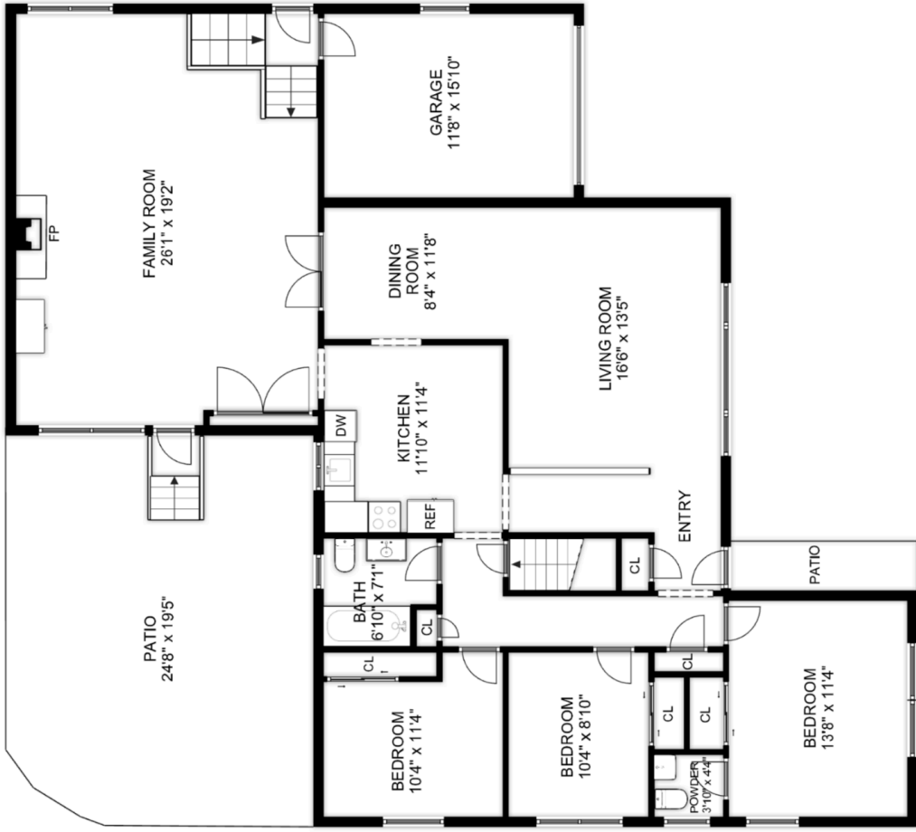
FIRST FLOOR
