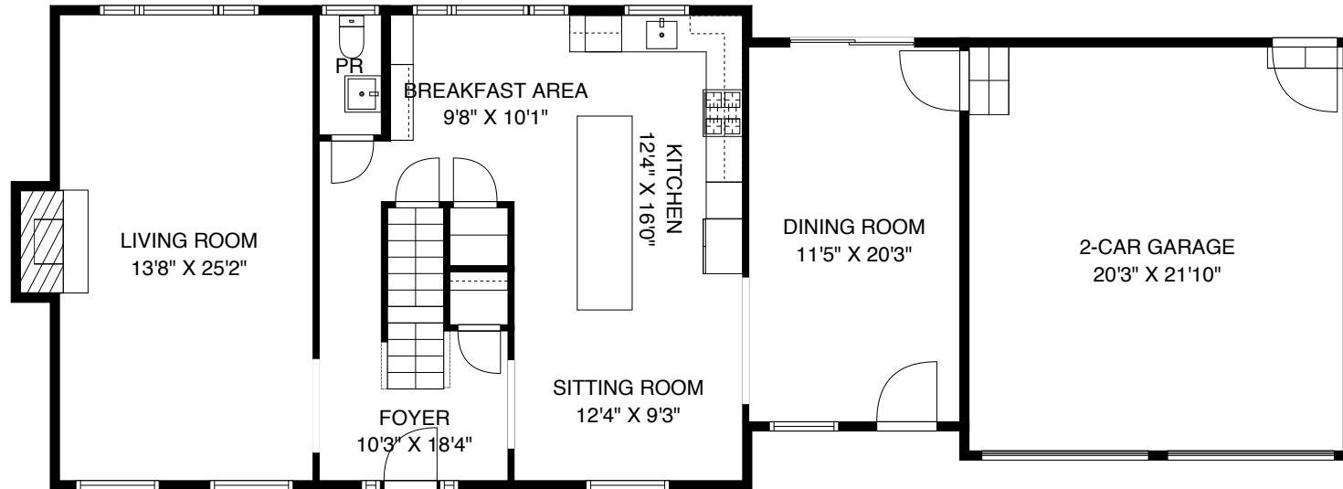
FIRST FLOOR
