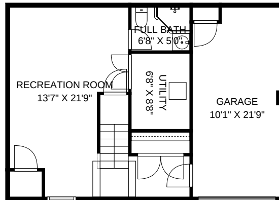
LOWER LEVEL
